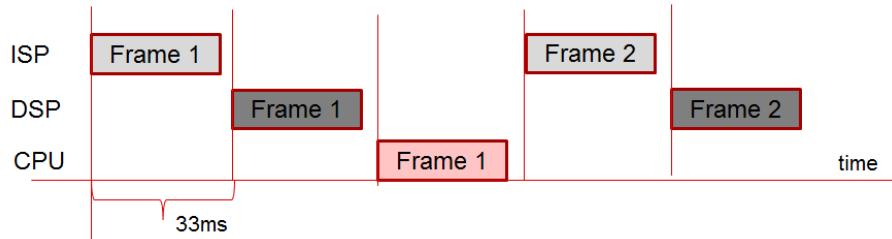
Figure 1.2: Non-pipelined Execution
