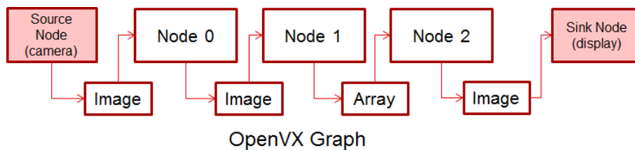
Figure 1.5: Source/Sink Nodes added for Graph Streaming
