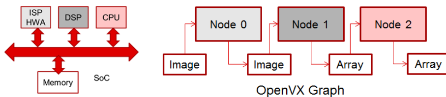
Figure 1.1: Example SoC and Distributed Graph
