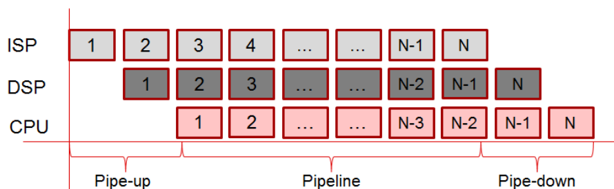
Figure 2.1: 3 Phases of pipeline: pipe-up, pipeline, and pipe-down
