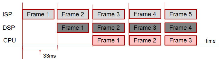
Figure 1.3: Frame-Level Pipelined Execution
