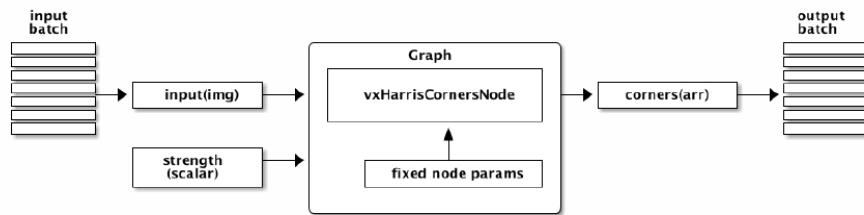
Figure 1.4: Graph Batch Processing
