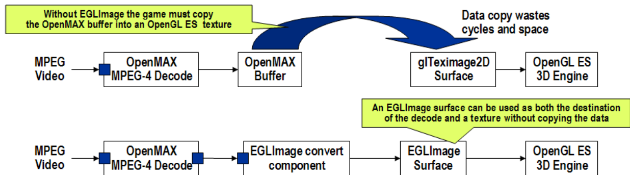
Figure 9: EGL 1.5 will enable efficient integration of video and graphics processing
