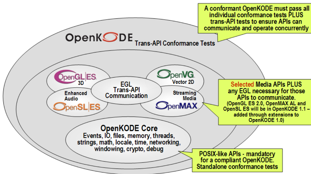
Figure 5: Components within an OpenKODE implementation
